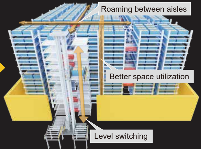
Goods-to-person Picking with Shuttle System
